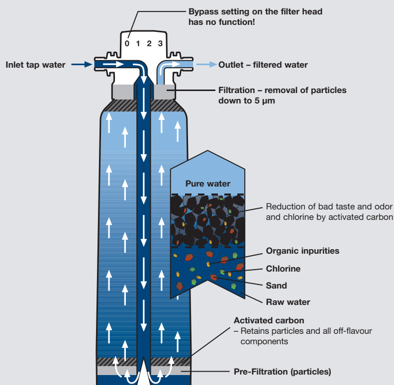
Cross-Section of a BWT besttaste filter cartridge
